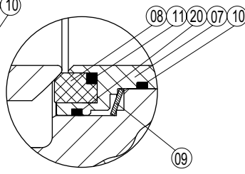
DETAIL A GRAFOIL \leq 350^{\circ}C
