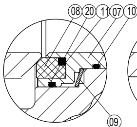
DETAIL A VITON \leq 200^{\circ}C
